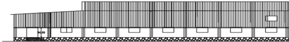
FRONT ELEVATION SCALE 1:100
